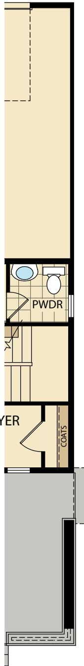
FIRST FLOOR END UNIT
