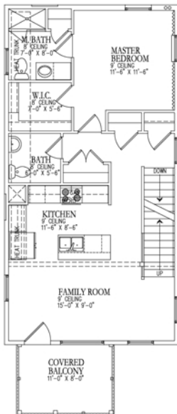
UPPER LEVEL 1
