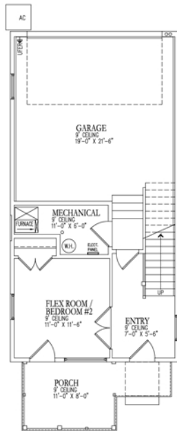
MAIN LEVEL
