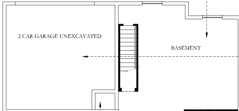
BASEMENT FLOORPLAN
