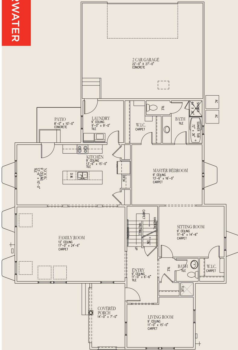
MAIN LEVEL
