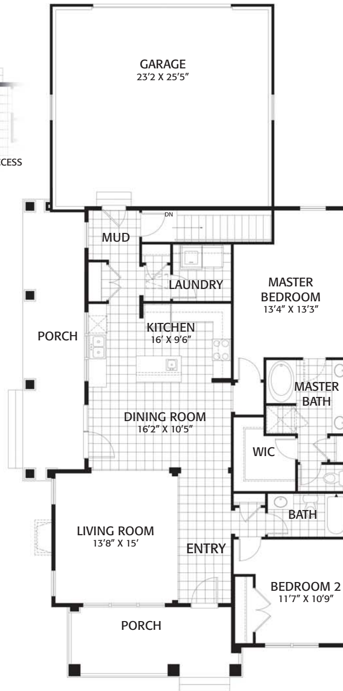
MAIN LEVEL
